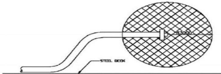
FIGURE-3 HORIZONTAL BALL OR PIG LAUNCHING OR RECEIVING INSTALLATION (N.T.S.) H 2 PURGED
