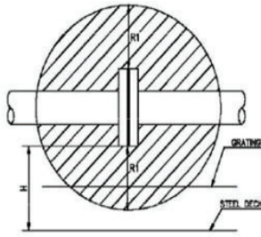
FIGURE-2A TYPICAL AREA CLASSIFICATION AROUND THE FLANGE/ VALVES INSTALLED OVER GRATED DECK IF INSTALLED OVER STEEL DECK H 2 (R1=1000mm)
