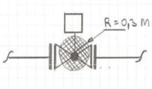
FIGURE-3 HORIZONTAL BALL OR PIG LAUNCHING OR RECEIVING INSTALLATION (N.T.S.) H 2 PURGED
