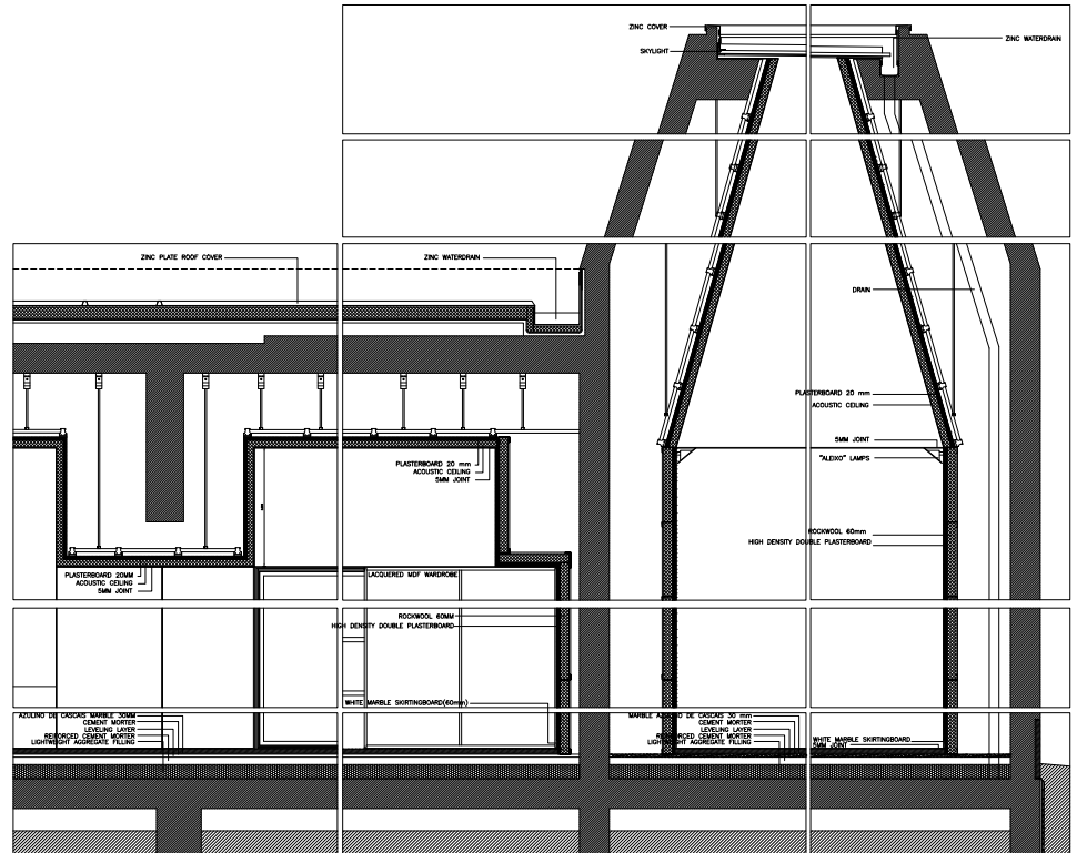
CONSTRUCTIVE SECTION 2 0 0.5 1m
